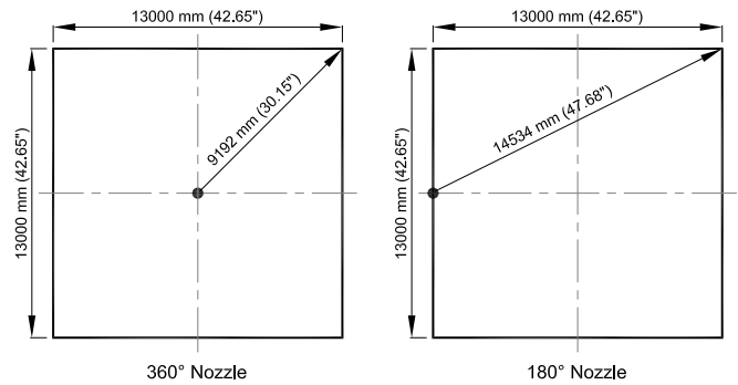
360° NOZZLE
